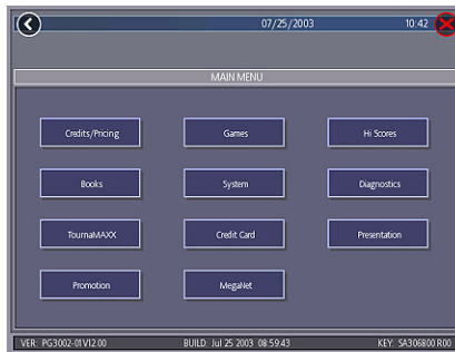
FIGURE 1 - MAIN MENU
