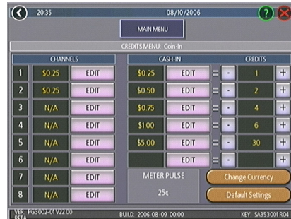
FIGURE 3 - COIN-IN MENU
