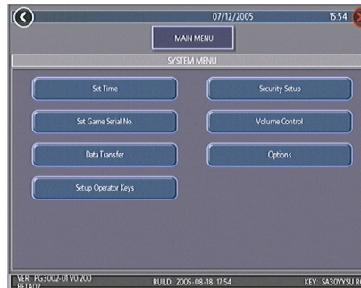
FIGURE 14 - SYSTEM MENU
