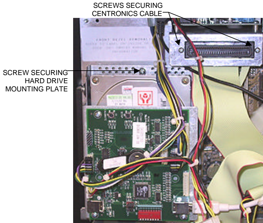
FIGURE 1 - MOTHERBOARD REMOVAL
