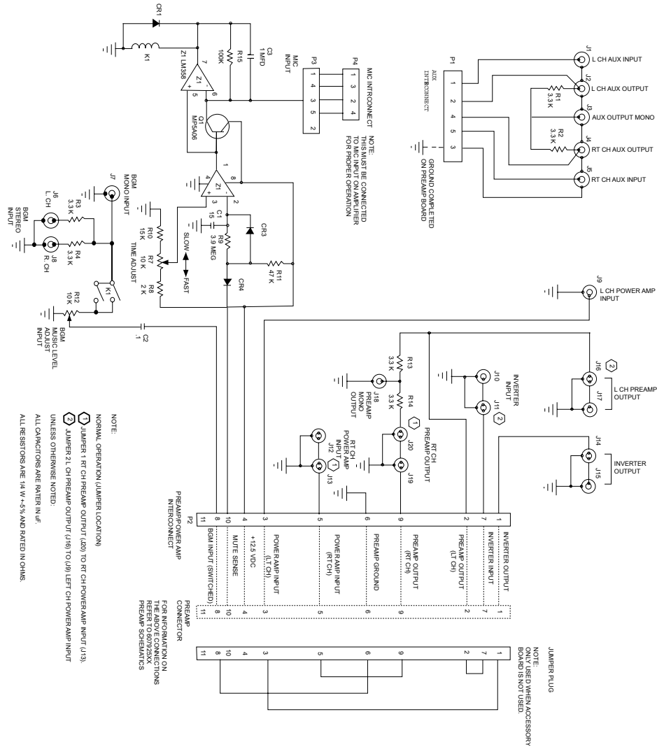
FIGURE 14 - ACCESSORY BOARD SCHEMATIC DIAGRAM
