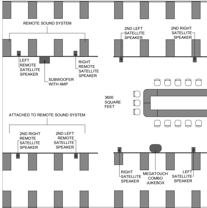
FIGURE 2 - BAR/RESTAURANT SOUND SYSTEM LAYOUT
