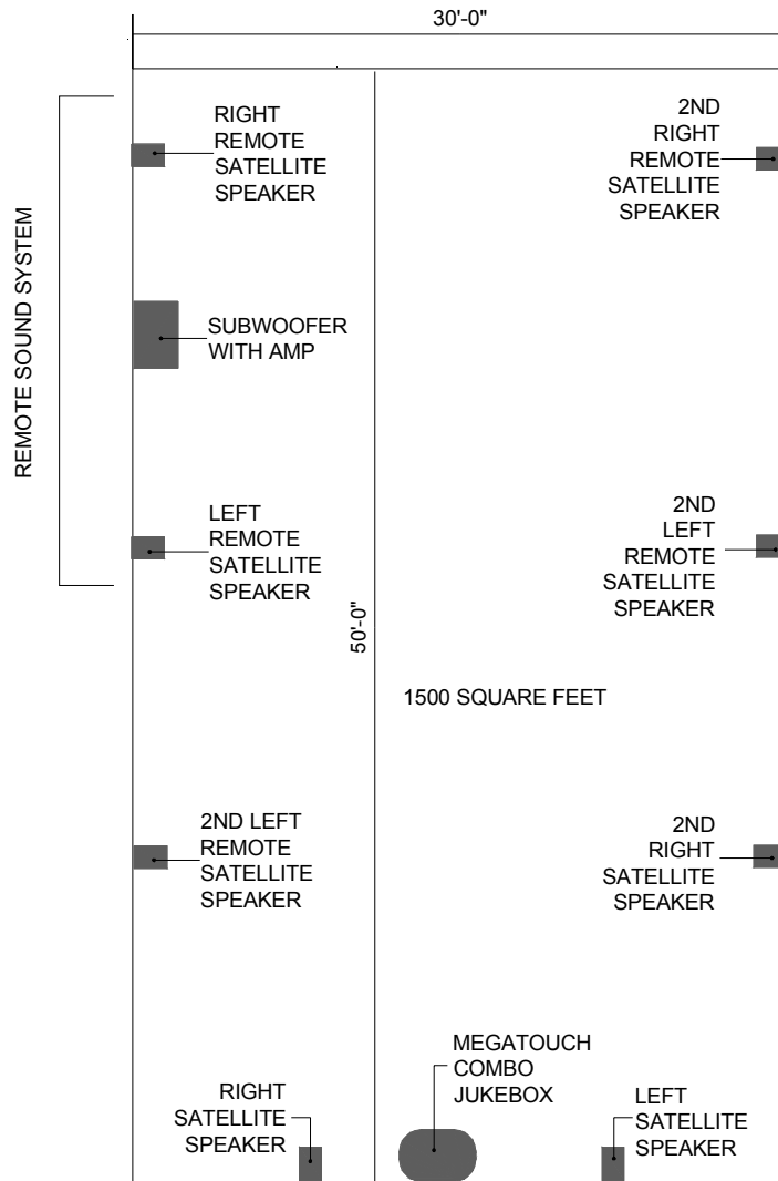
FIGURE 4 - LARGE RECTANGLE ROOM (2) SOUND SYSTEM LAYOUT
