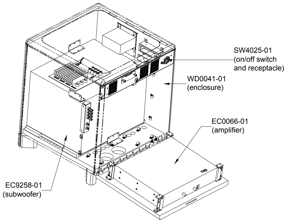
FIGURE 1 - REMOTE SOUND SYSTEM CABINET
