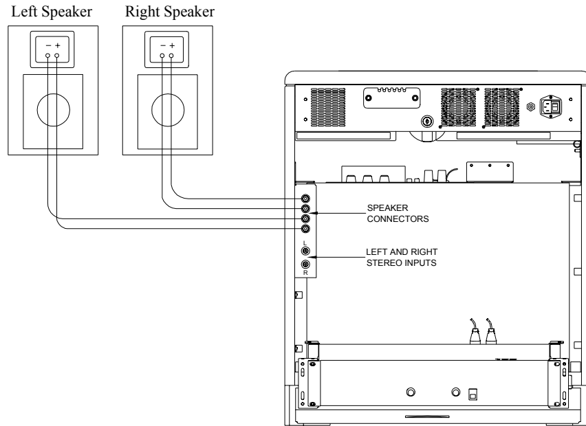
FIGURE 6 - REMOTE SOUND SYSTEM AUDIO CONNECTIONS
