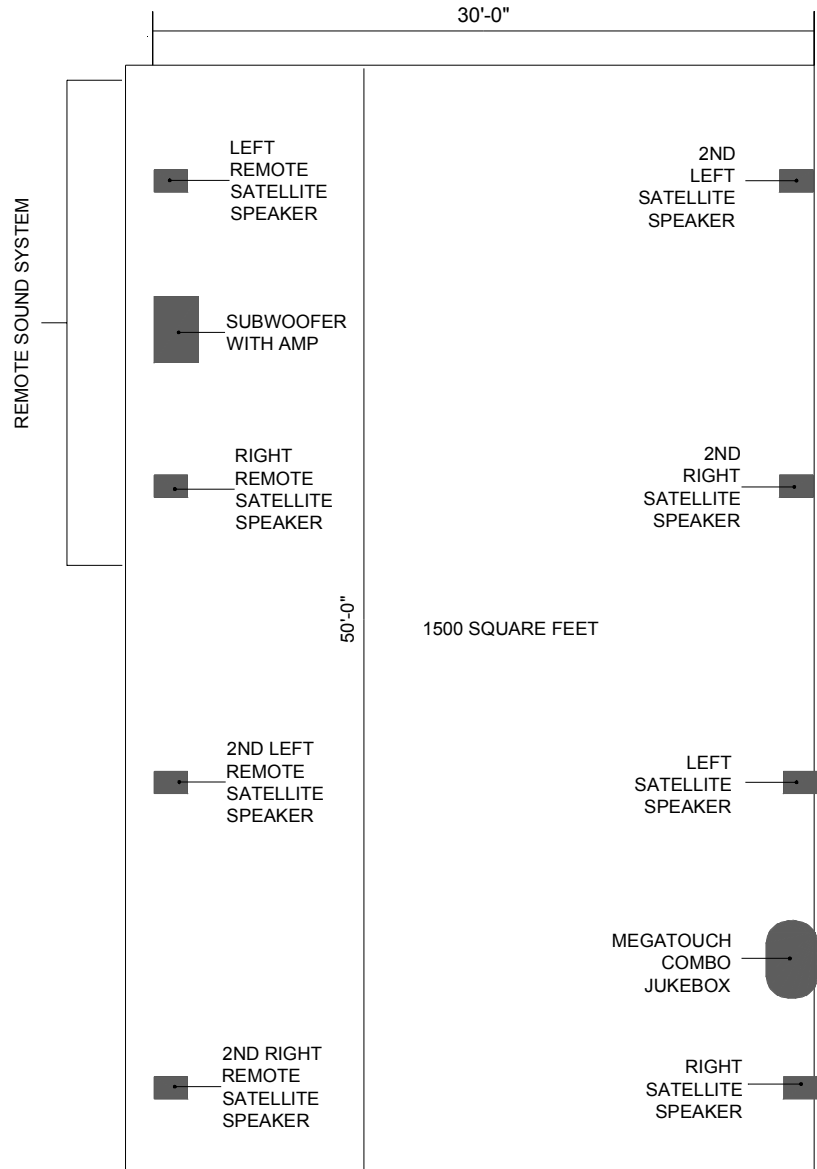
FIGURE 3 - LARGE RECTANGLE ROOM (1) SOUND SYSTEM LAYOUT
