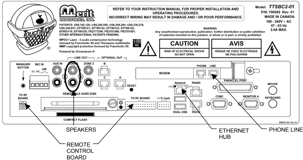
FIGURE 7 - SINGLE BOARD COMPUTER CONNECTIONS
