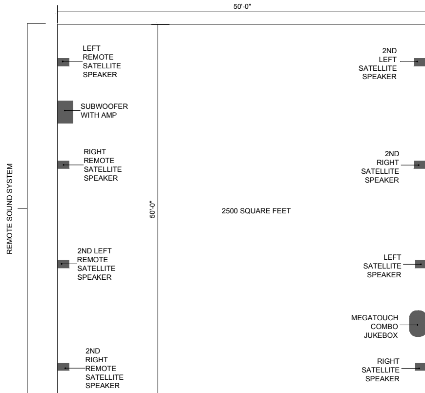
FIGURE 5 - LARGE SQUARE ROOM SOUND SYSTEM LAYOUT
