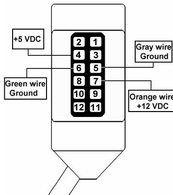
TOUCHSCREEN OVERLAY CONNECTOR
