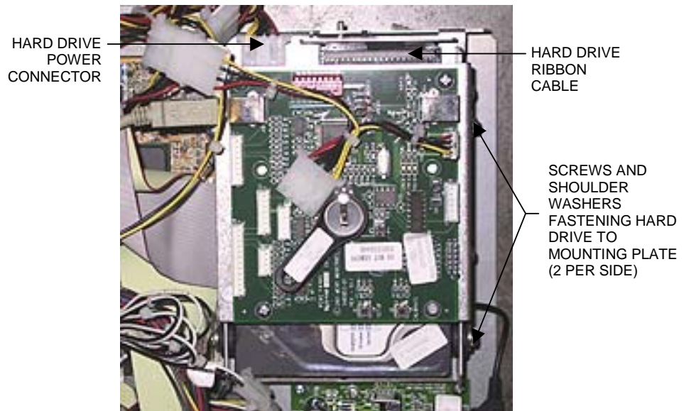
FIGURE 3 - CLOSEUP OF HARD DRIVE
