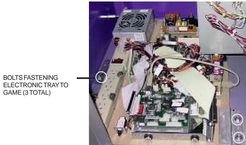
FIGURE 2 - CPU SECTION - ELECTRONICS TRAY MOUNTED ON BOTTOM WALL
