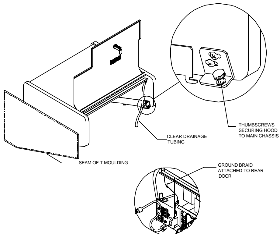
FIGURE 2 - HOOD ASSEMBLY T-MOULDING PULLED AWAY FROM GAME
