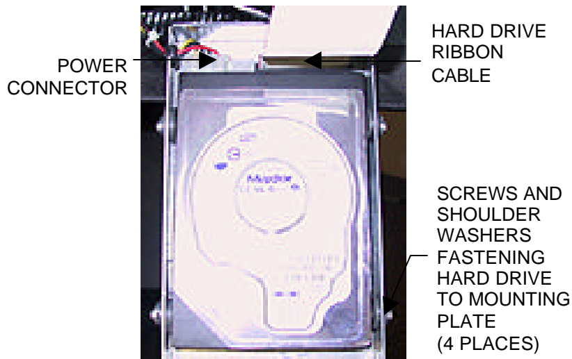
FIGURE 1 - BLUE MAXX/MAXX CLASSIC - CLOSEUP OF HARD DRIVE
