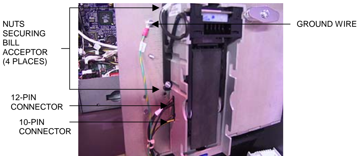
FIGURE 1 - OPEN CASH DOOR AND BILLACCEPTOR
