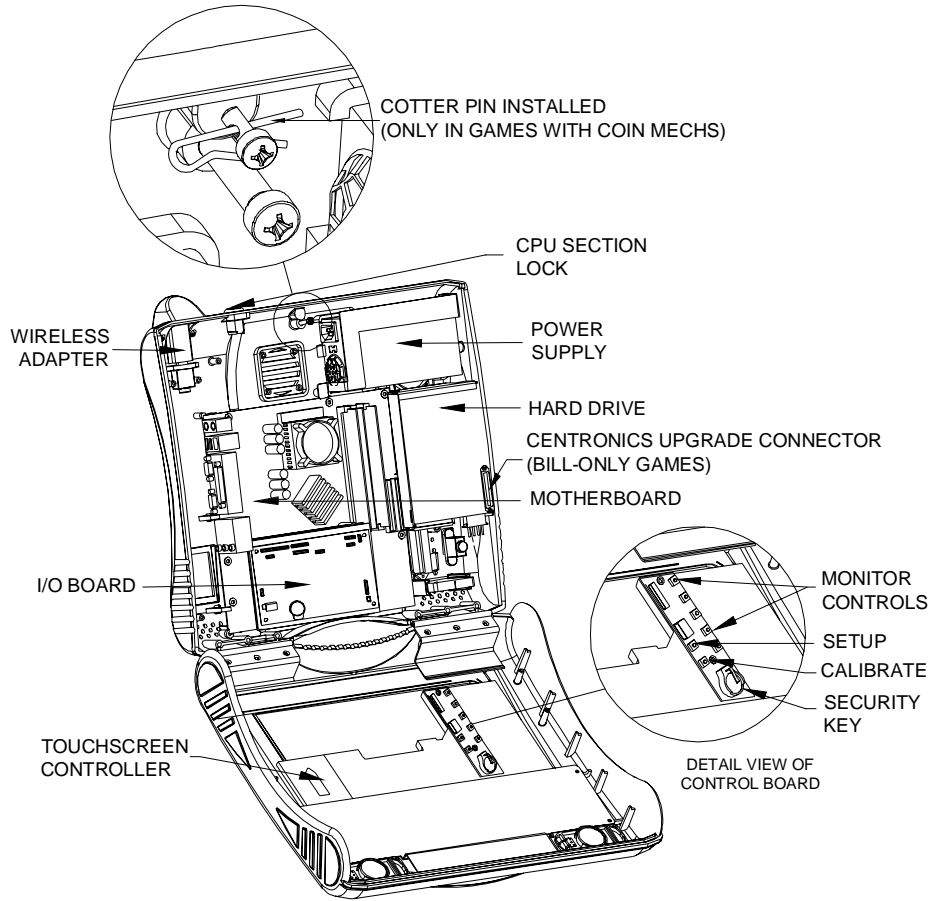
FIGURE 30 - CPU SECTION
