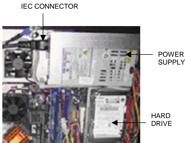
FIGURE 1 - OVERVIEW OF HARD DRIVE
