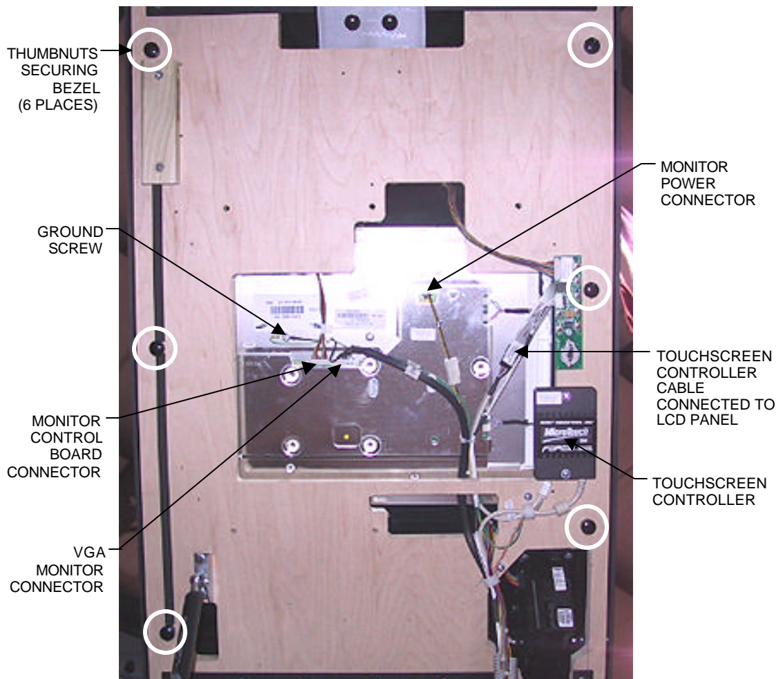
FIGURE 1 - UNDERSIDE OF BEZEL
