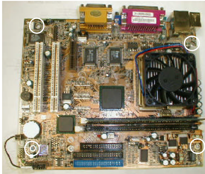
FIGURE 1 – MOTHERBOARD REMOVAL – LOCATION OF SCREWS SECURING MOTHERBOARD TO CPU SHELF
