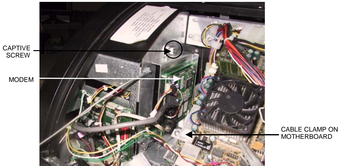
FIGURE 7 - MODEM IN GAME
