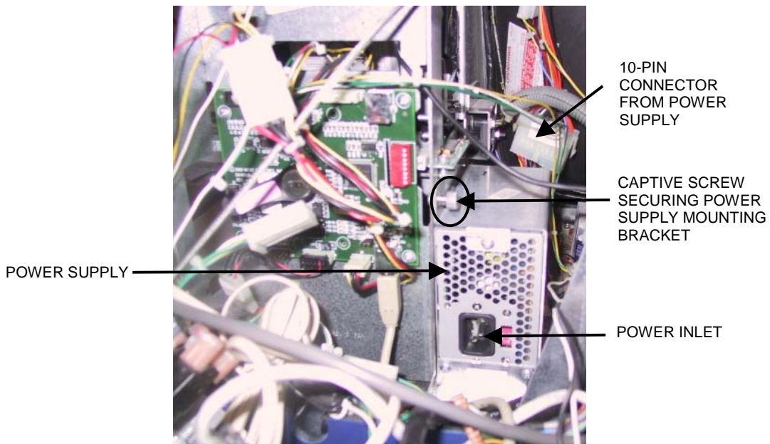
FIGURE 8 - POWER SUPPLY IN GAME
