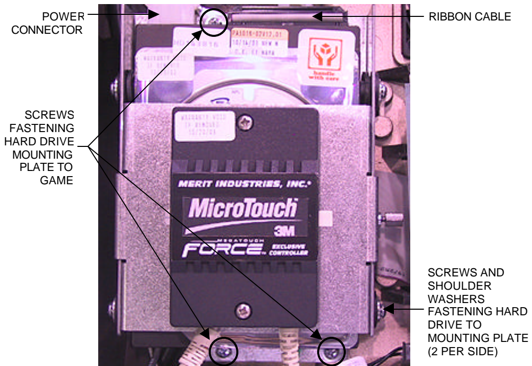
FIGURE 1 - SCREWS FASTENING HARD DRIVE MOUNTING PLATE TO GAME
