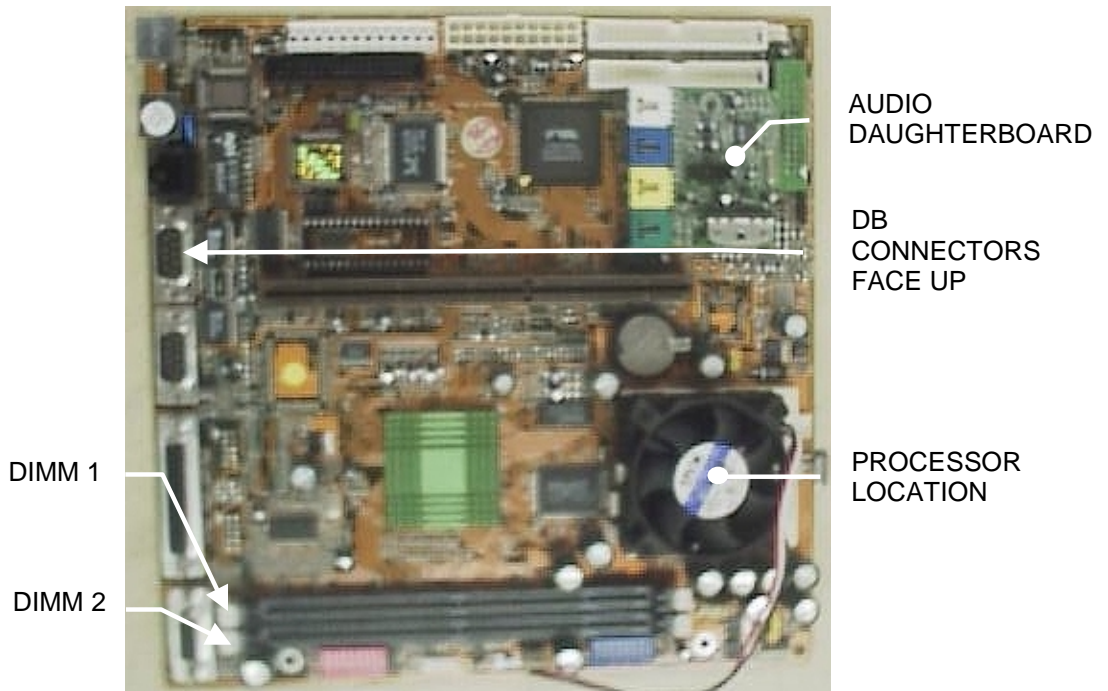
FIGURE 4B - UNICORN 586 MOTHERBOARD WITH I/O AND RISER REMOVED
