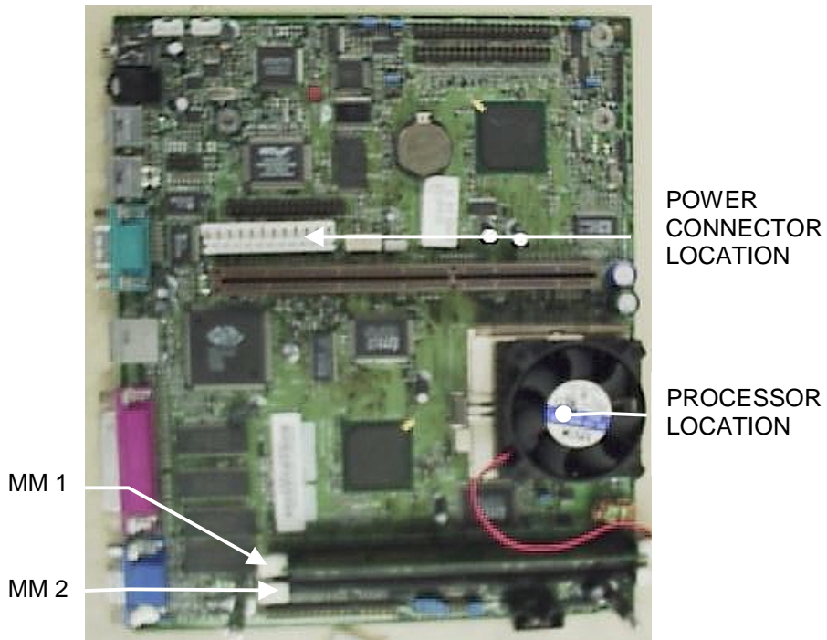
FIGURE 3B - ITOX 586 MOTHERBOARD WITH I/O AND RISER REMOVED
