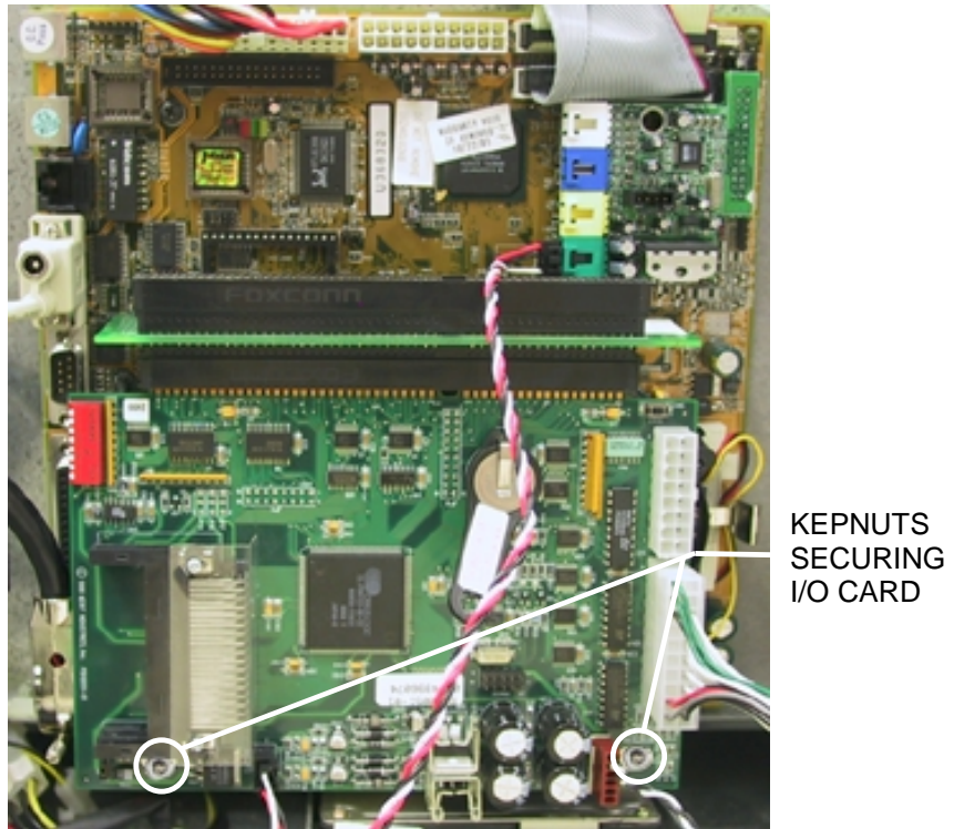
FIGURE 4A - UNICORN 586 MOTHERBOARD
