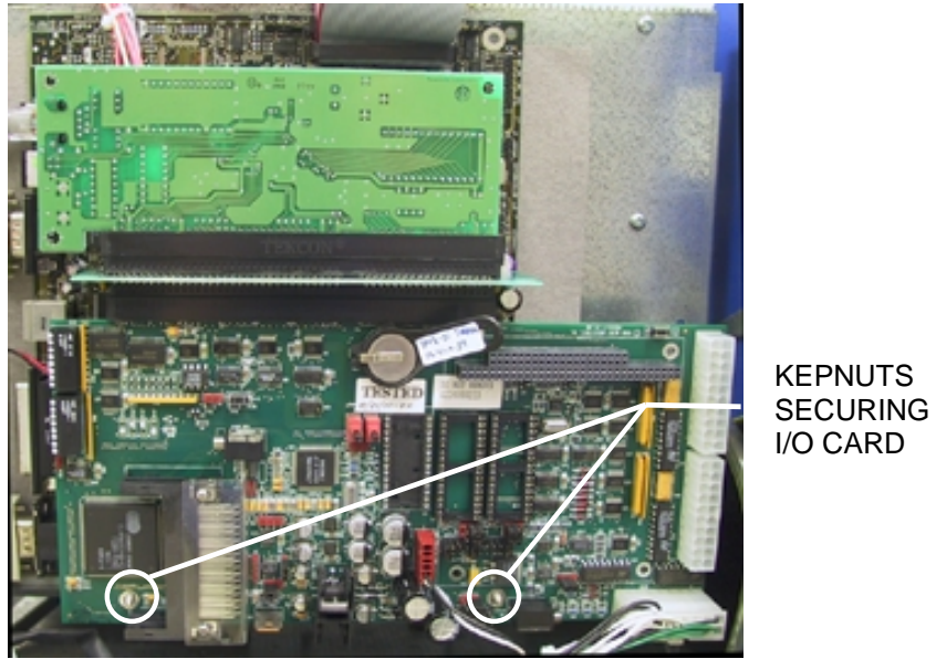
FIGURE 2A - MITSUBISHI 586 MOTHERBOARD
