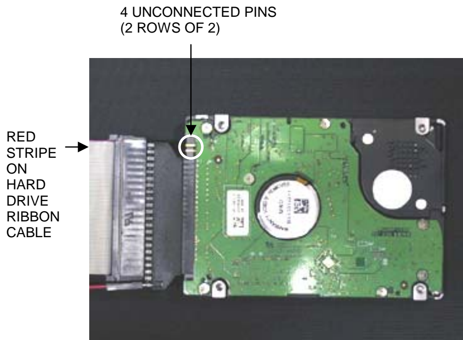
FIGURE 2 - CIRCUIT-BOARD SIDE OF HARD DRIVE
